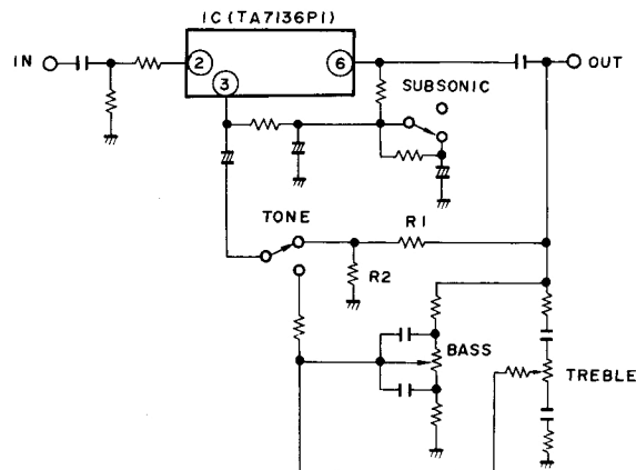
Fig. 4-2 Tone control circuit
