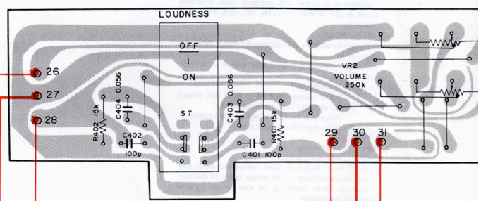
VOLUME Ass'y GWX-322
