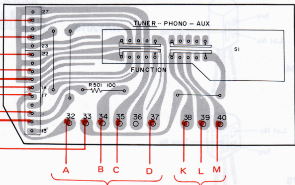
SWITCH Ass'y GWX-321
