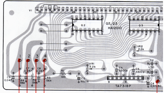
INDICATOR Ass'y AUV-004
