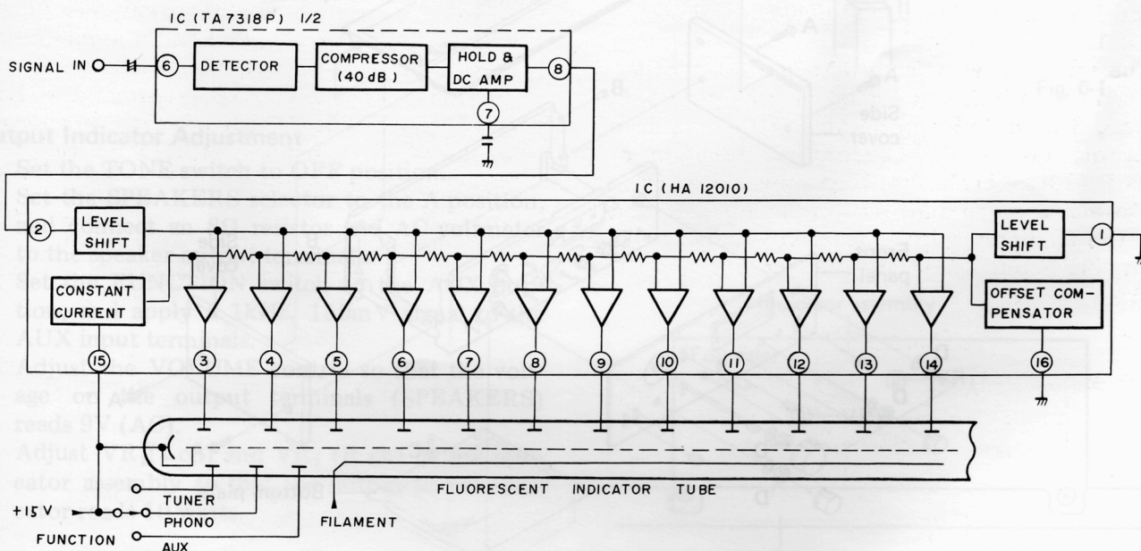
Fig. 4-4 Indicator circuit
