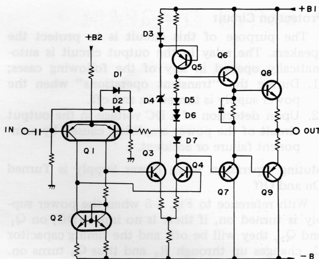
Fig. 4-3 Power amplifier
