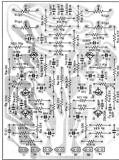
Control amp ass'y AWR-008
