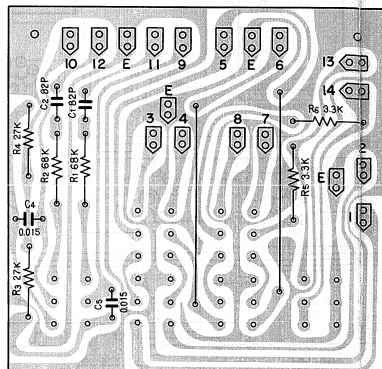
Switch circuit ass'y AWS-014
