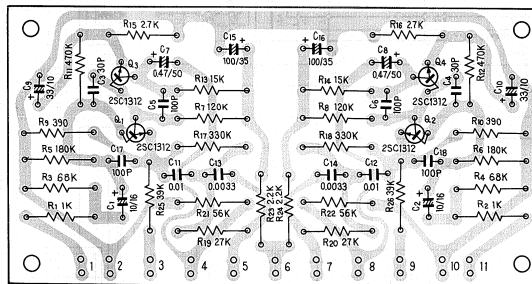
Equalizer amp ass'y W21-004
