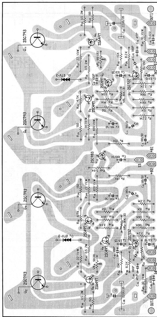
Power amp ass'y AWH-002
