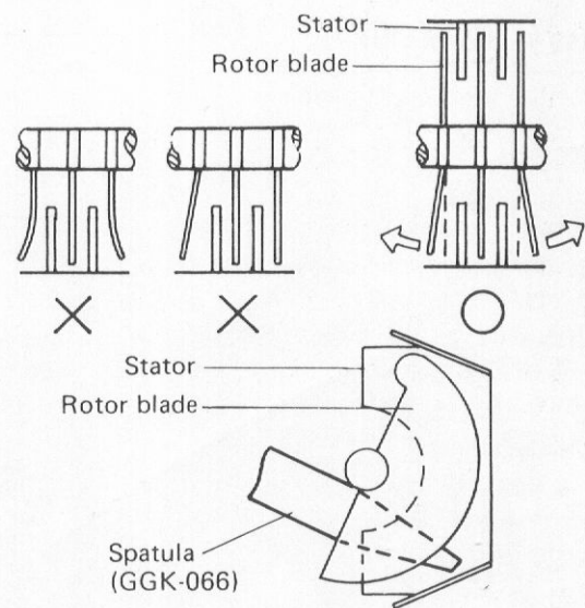
Fig. 8-3 Adjustment of Tuning Capacitor
