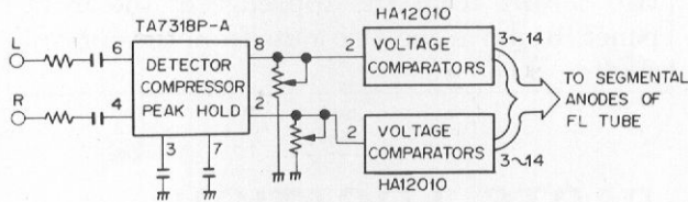
Fig. 4-3 Power Indicator Circuit
