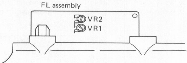
Fig. 8-2 Power Indicator Calibration
