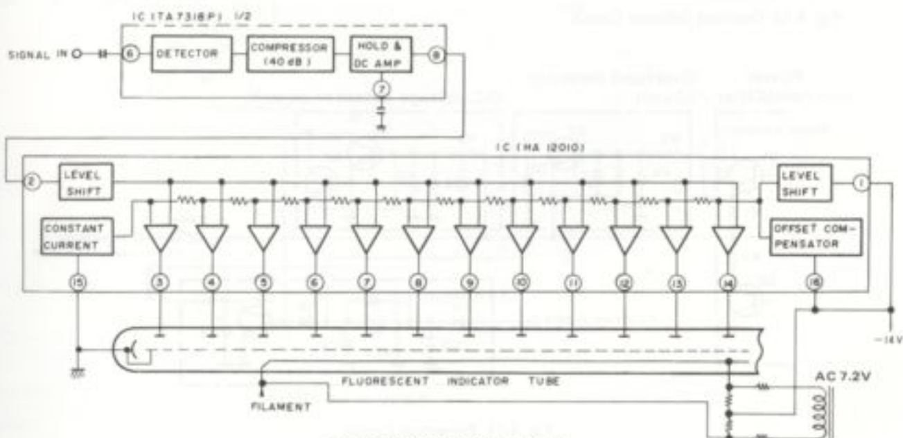
Fig. 4-9 Power indicator circuit
