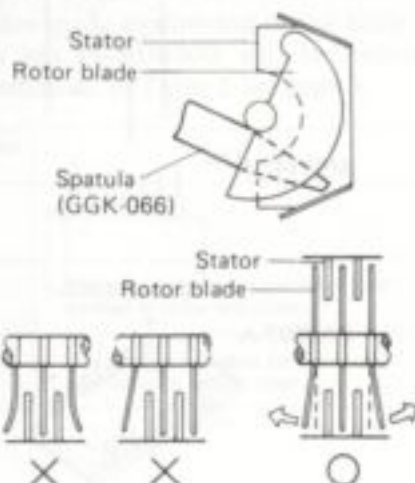
Fig. 8-1 Adjustment of tuning capacitor
