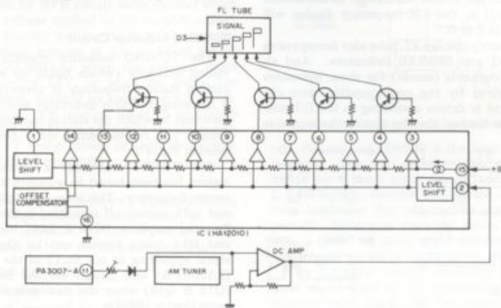
Fig. 4-8 SIGNAL indicator driver circuit
