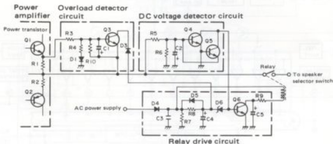
Fig. 4-11 Protection Circuit
