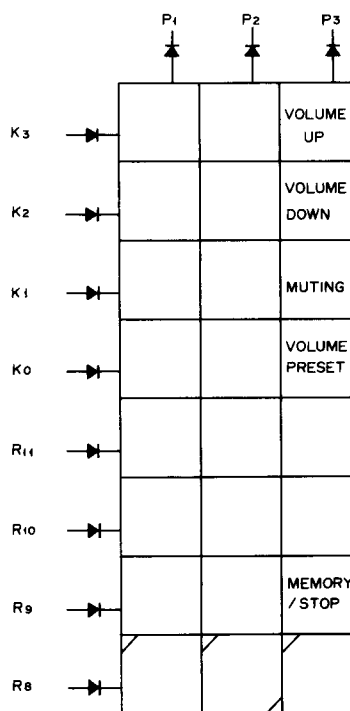
Fig. 1-7 Switch key matrix for volume control
