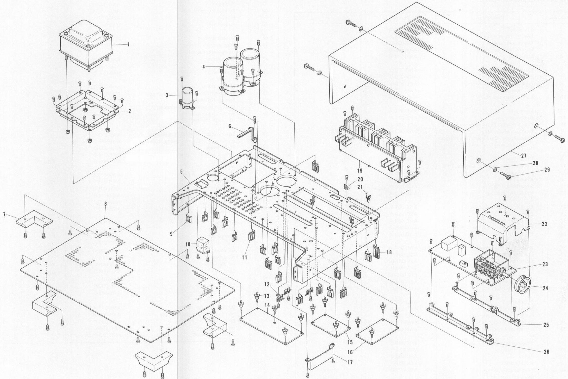
Exploded View-1
