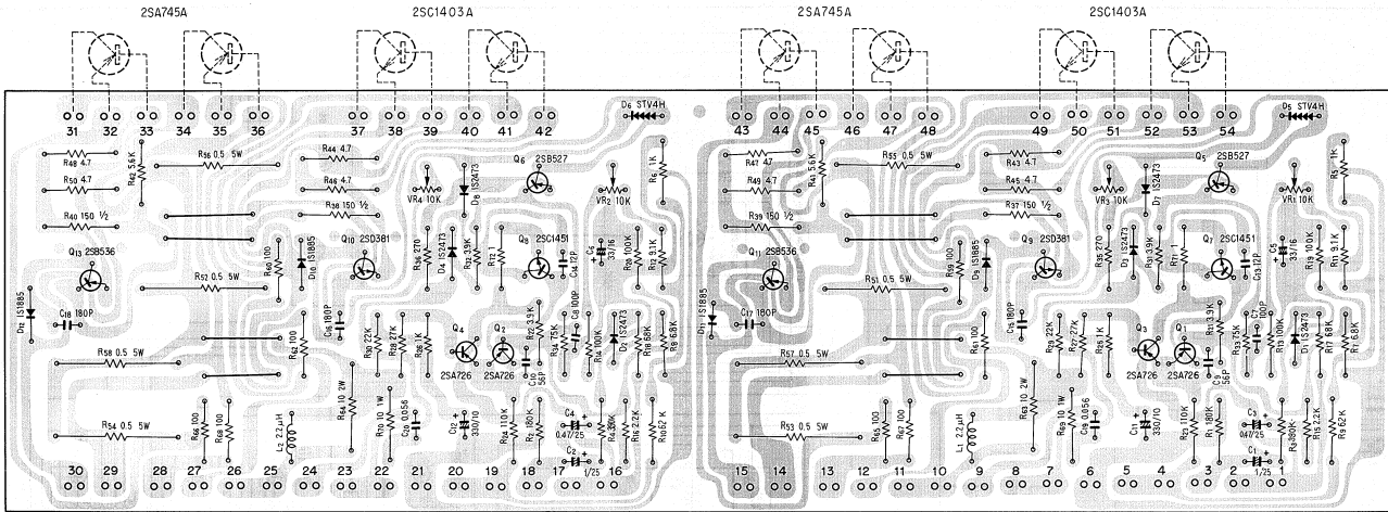
Power amp ass'y AWH-030
