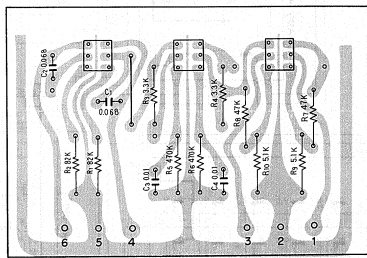
Switch circuit ass'y AWS-066
