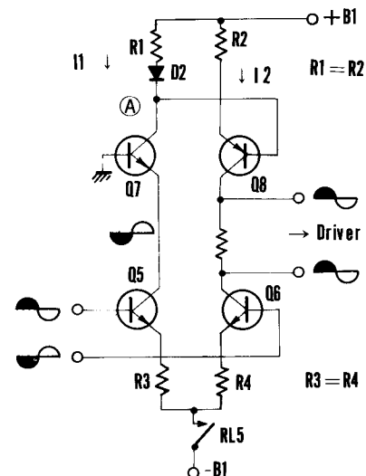
Fig. 1 Current Mirror Circuit
