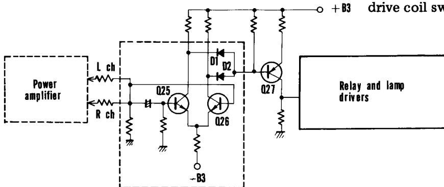
Fig. 10 DC Balance Detector Circuit
