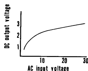
Fig. 5 Input-output Response
