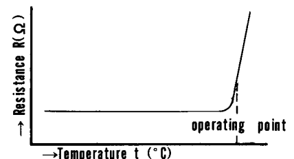
Fig. 8 Posistor-temperature Response
