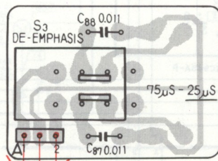
DE-EMPHASIS Ass'y GWS-188
