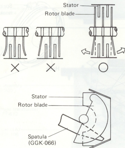
Fig. 8-1 Adjustment of tuning capacitor
