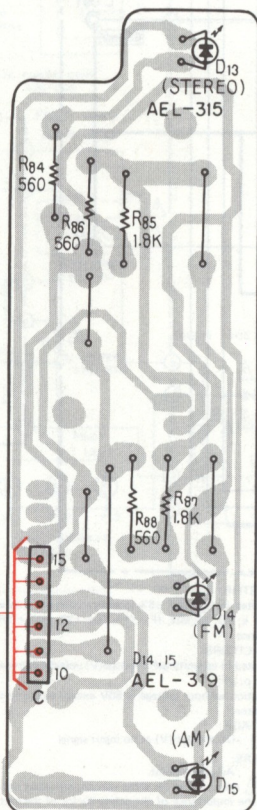
LED Ass'y GWX-308
