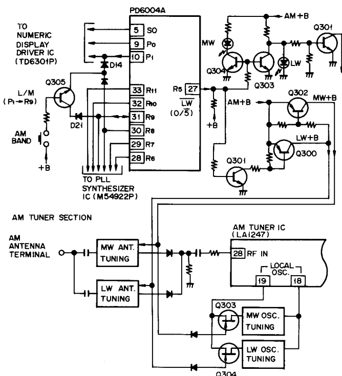
Fig. 6-11 MW/LW band selection for TX-930L
