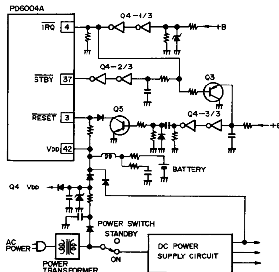
Fig. 6-16 Microcomputer back-up power supply
