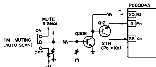
Fig. 6-8 Tuning mode selection of TX-930L
