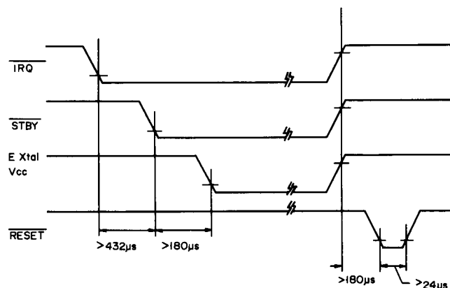
Fig. 6-17 Power supply sequence for stop/restart
