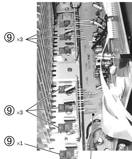
REGULATOR Assy
