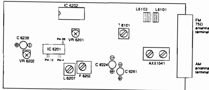
Fig. 1-2 Adjustment Points
