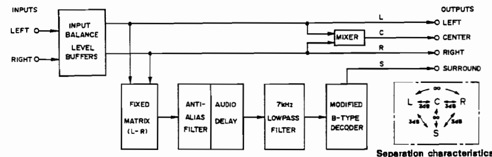
Figure 10-1. Block diagram of conventional Dolby surround circuit
