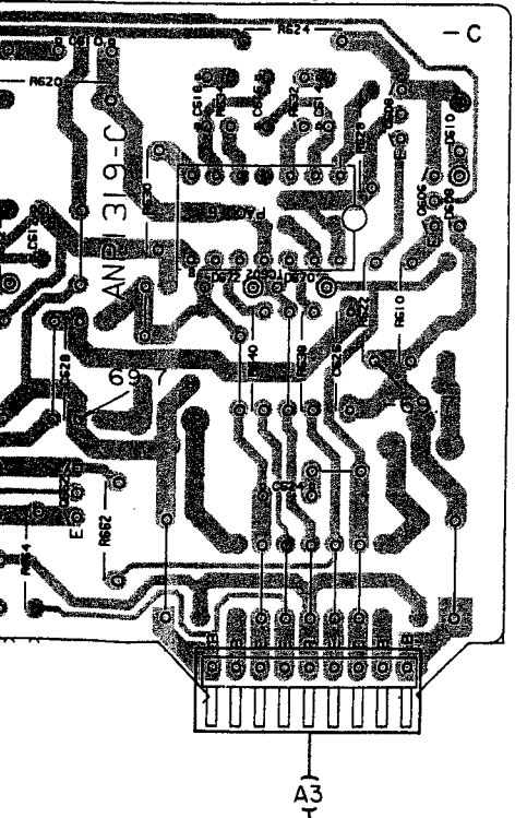
FRONT AMP assembly (AWH1014)
