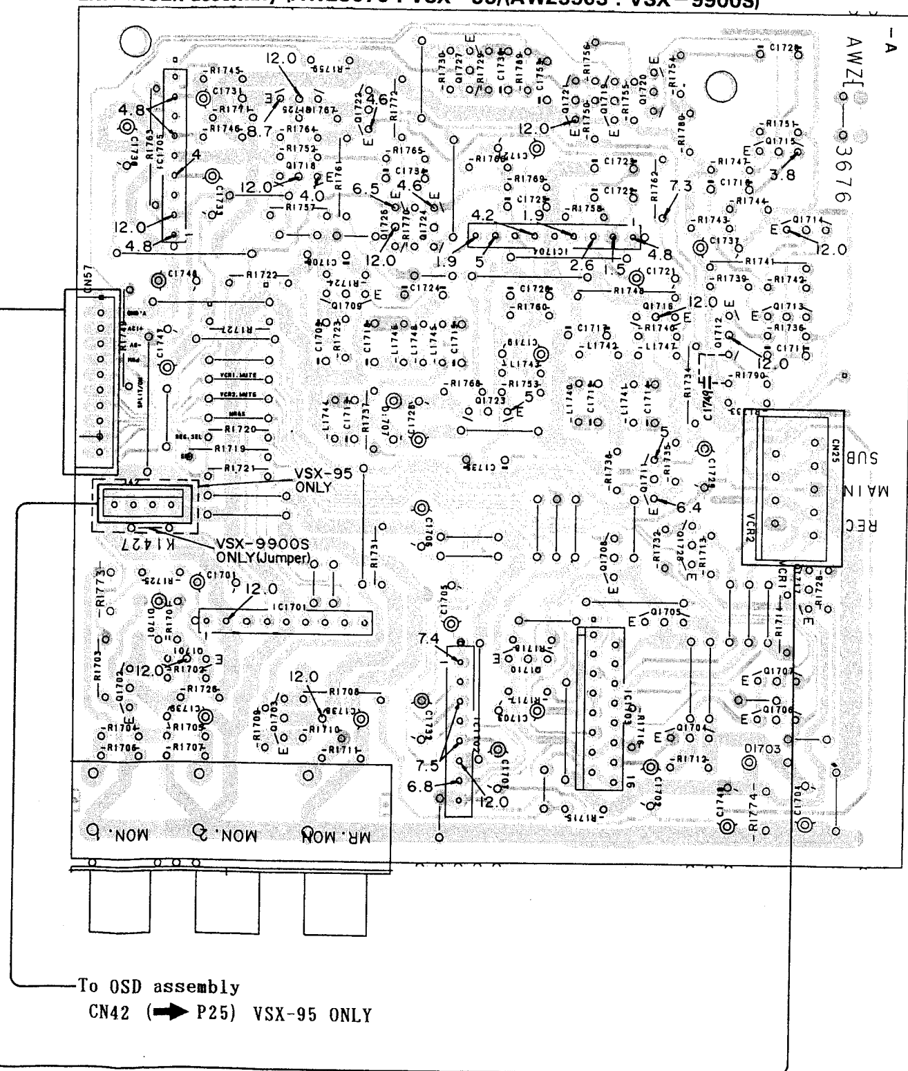
ENHANCER assembly (AWZ3676 : VSX-95) (AWZ3563 : VSX-9900S)
