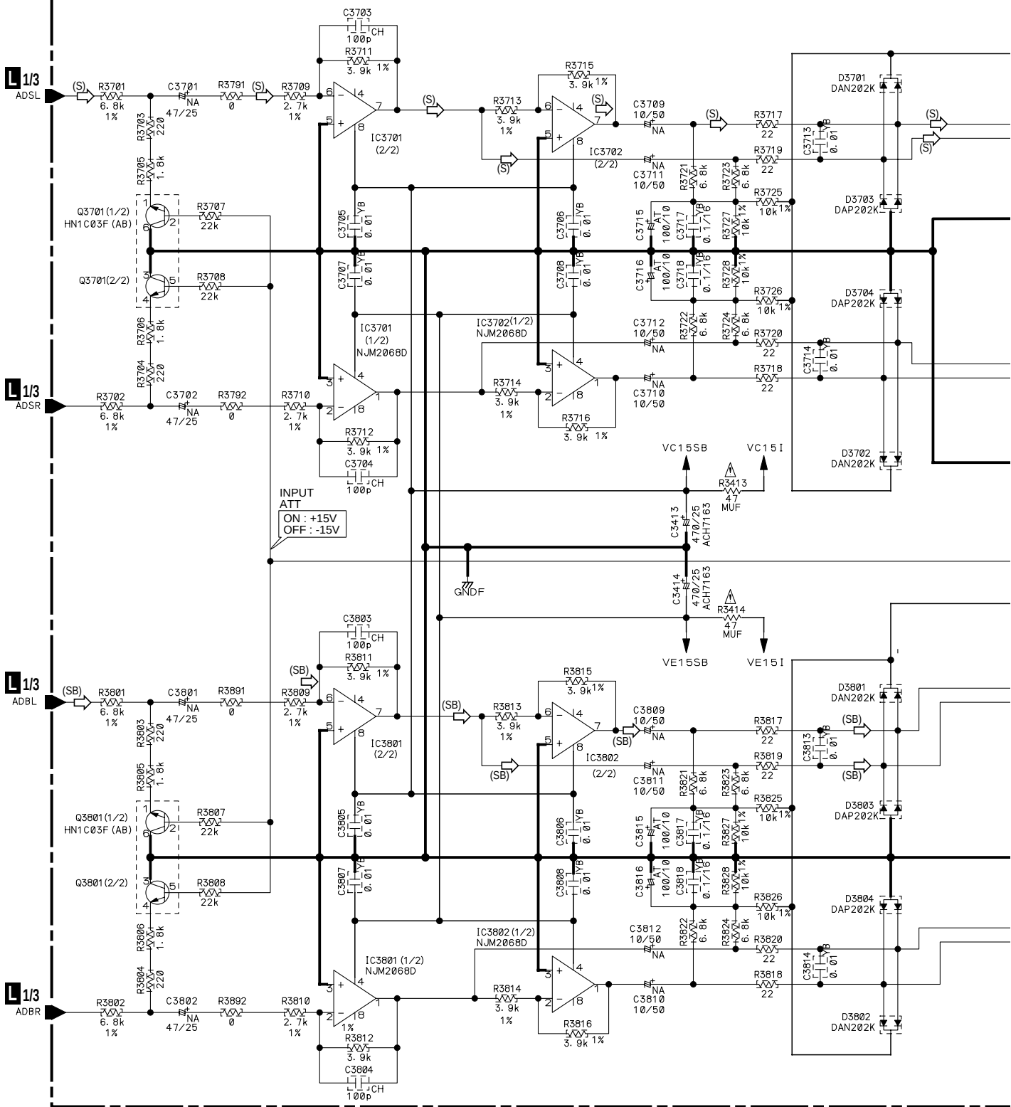
3/3 ANALOG IN & A/D ASSY (AWX7878)(VSX-49TX ONLY)
