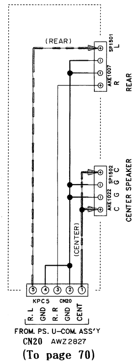
AWZ2836 R. C. SP. ASS'Y
