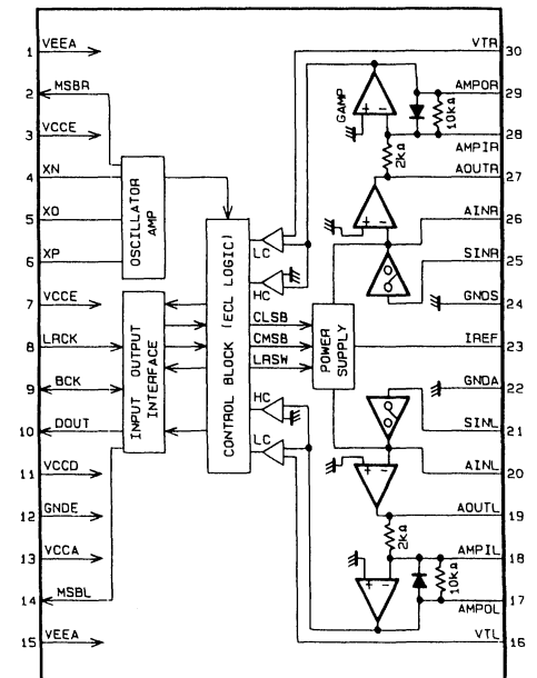
TD6726N DSP.U-COM. Ass'y (Page 21)
