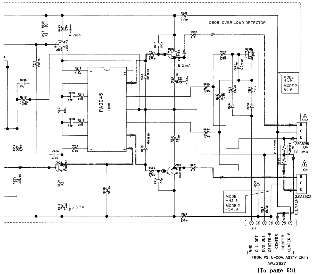
AWZ2836 R. C. SP. ASS'Y
