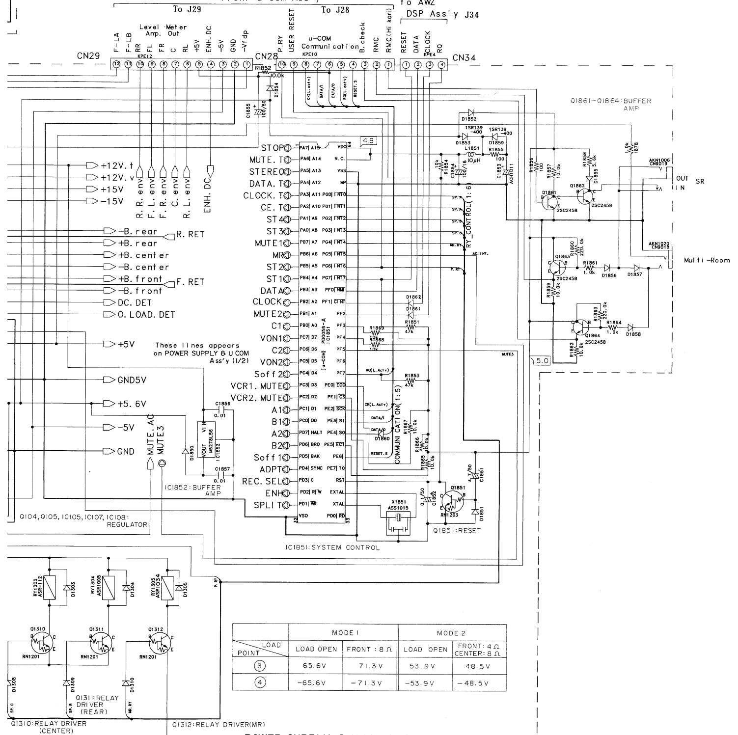
POWER SUPPLY &amp; U COM Ass'y(2/2) AWZ2827
