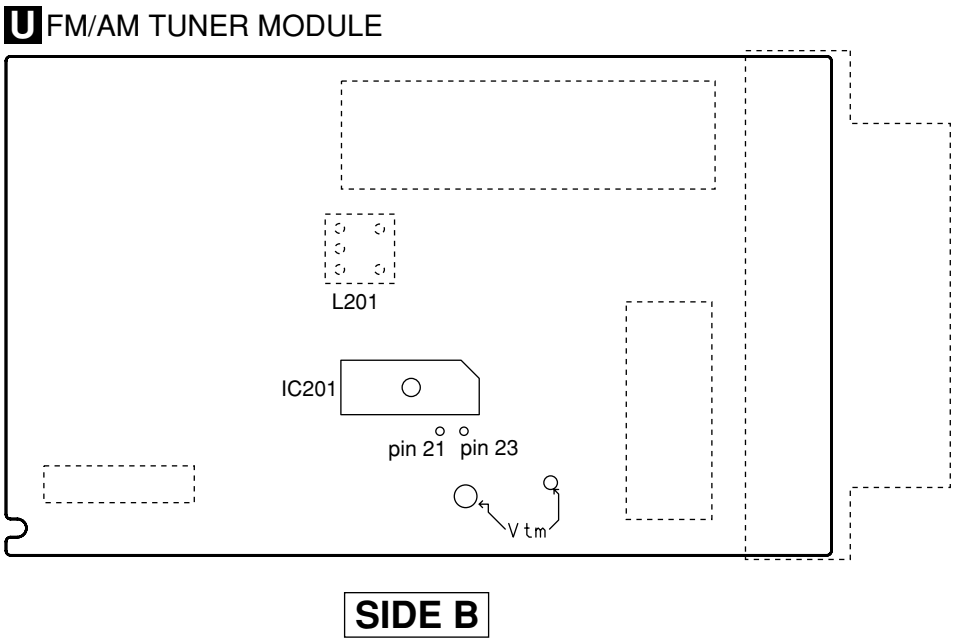
Fig.2 Adjustment Point
