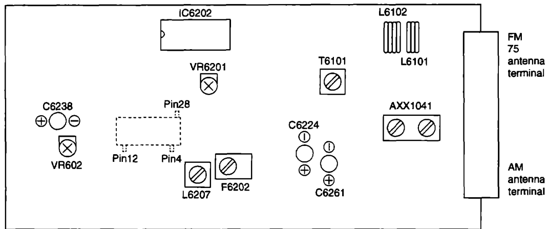
Fig. 1-2 Adjustment Points
