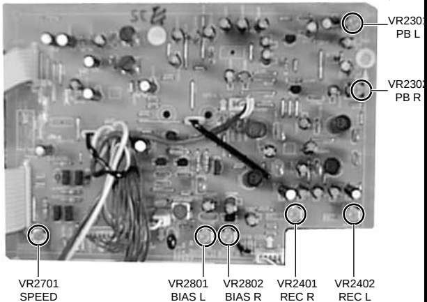
DECK Assy Adjustment Point
