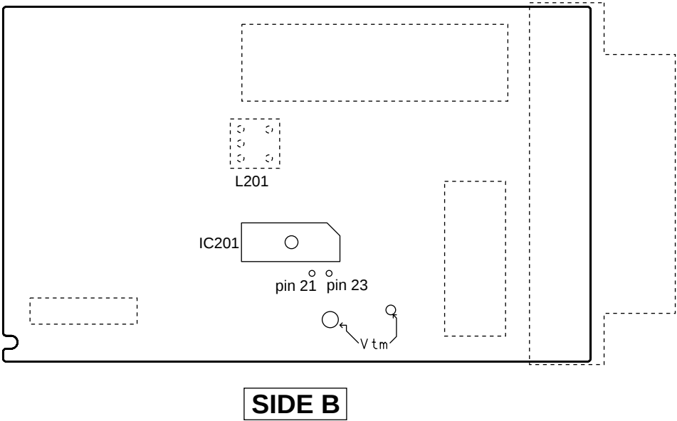
Fig.6.6 Adjustment Point
