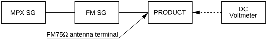
Fig.6.5 Adjustment Wiring Diagram
