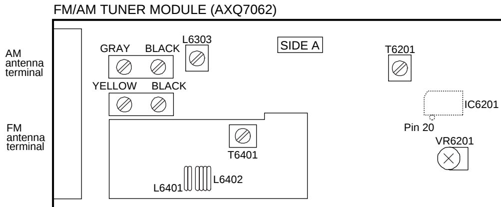
Fig. 4 Adjustment Point
