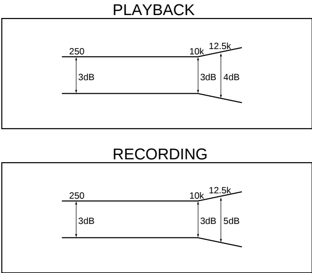
Fig. 8 Frequency Characteristics
