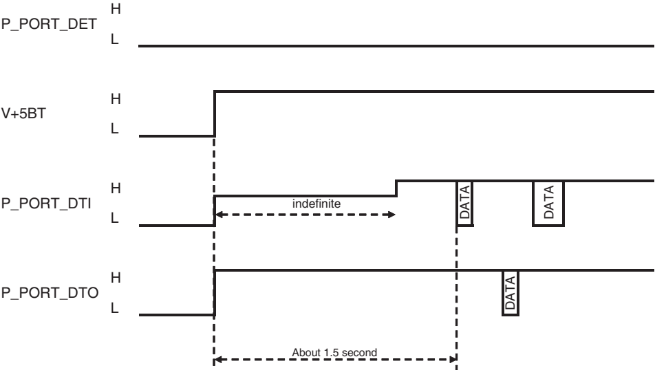
ADP_DET logic
