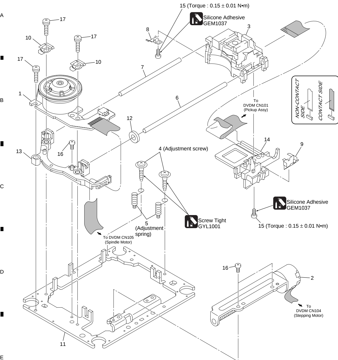
TRAVERSE MECHA ASSY-S parts List
