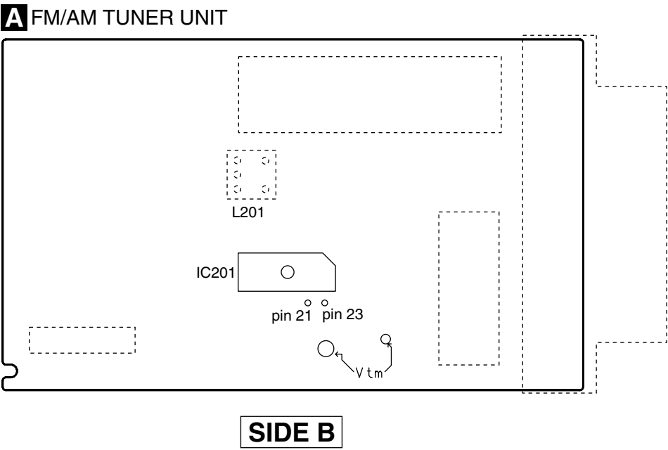
Fig.6.6 Adjustment Point E
