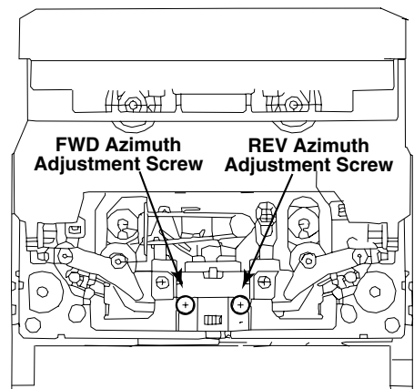
Fig. 6-3 Adjustment and Measurement Points
