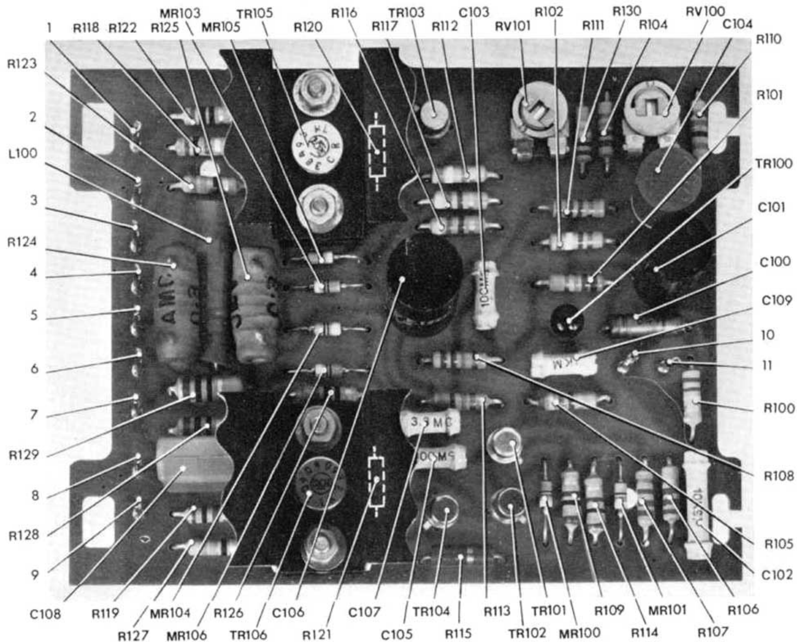
Fig. 11 (a) Driver Board M.12038 (issue 9)
