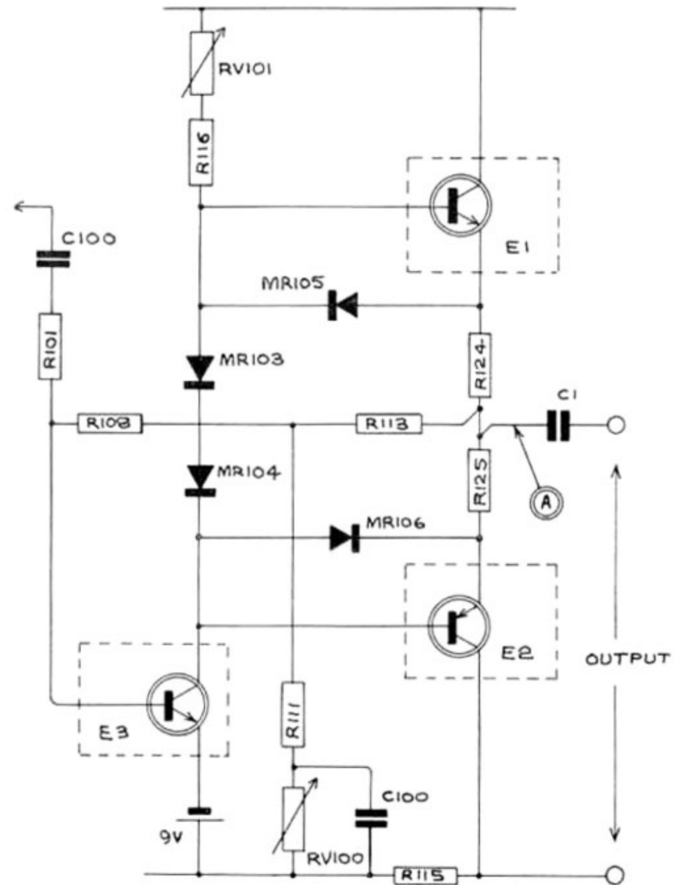
Fig. 2 Simplified circuit, Quad 303
