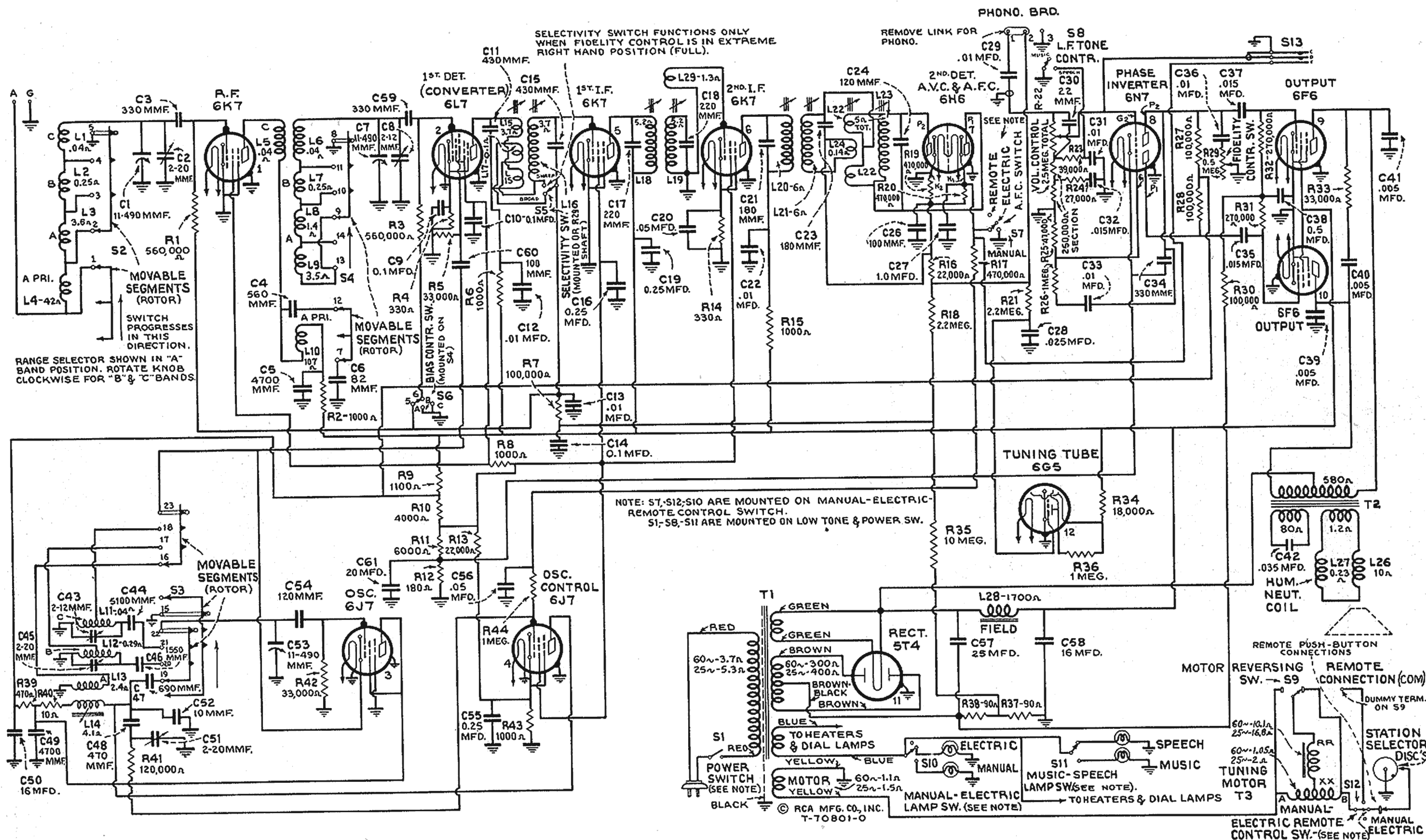
Figure 1—Schematic Circuit Diagram
