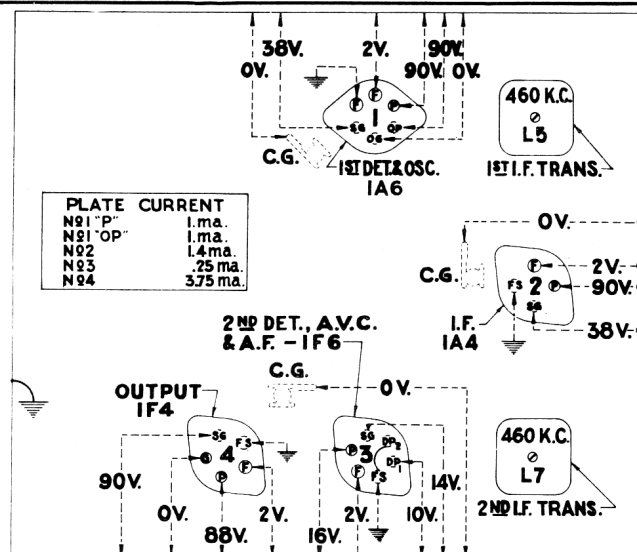
Figure 4—Radiotron Socket Voltages, Coil, and Trimmer Locations
