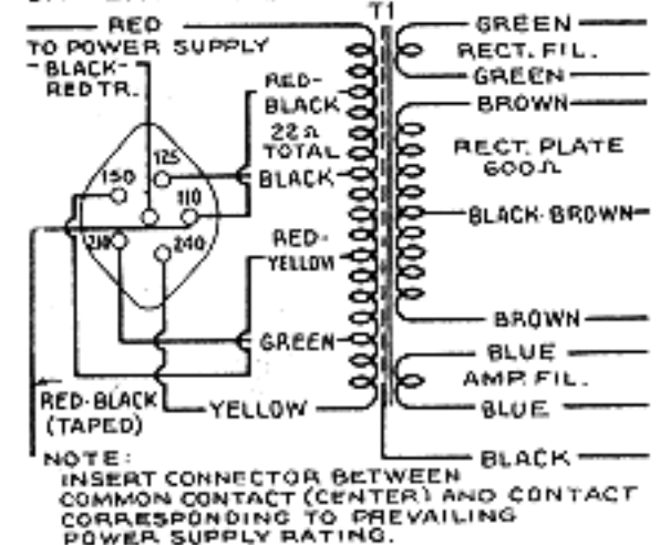
UNIVERSAL TRANSFORMER CONNECTIONS
