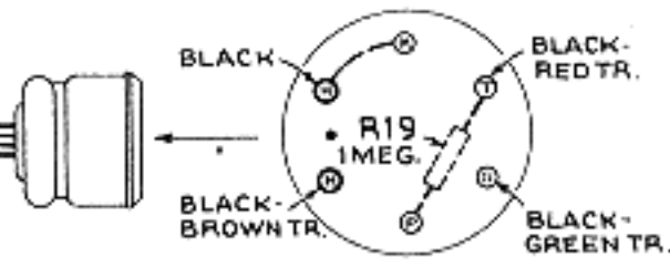
TUNING CABLE CONNECTIONS
