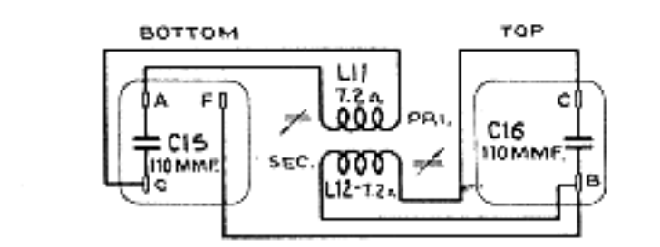
1ST. I.F. TRANS. CONNECTIONS
