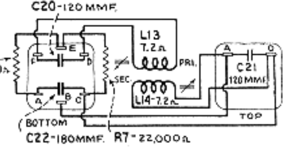
2ND. I.F. TRANS. CONNECTIONS
