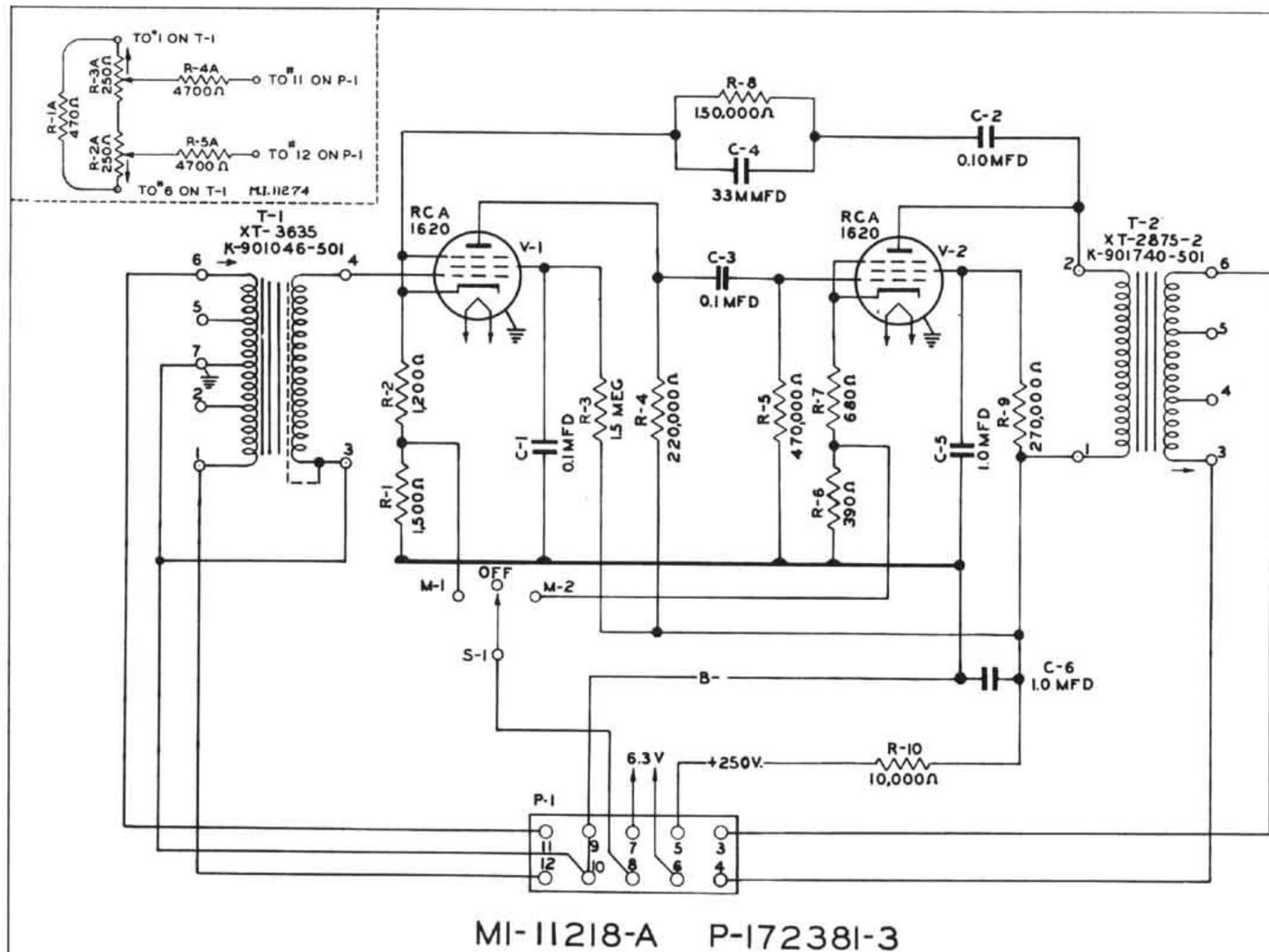
Figure 2—Schematic diagram of Type BA-1A Preamplifier.
