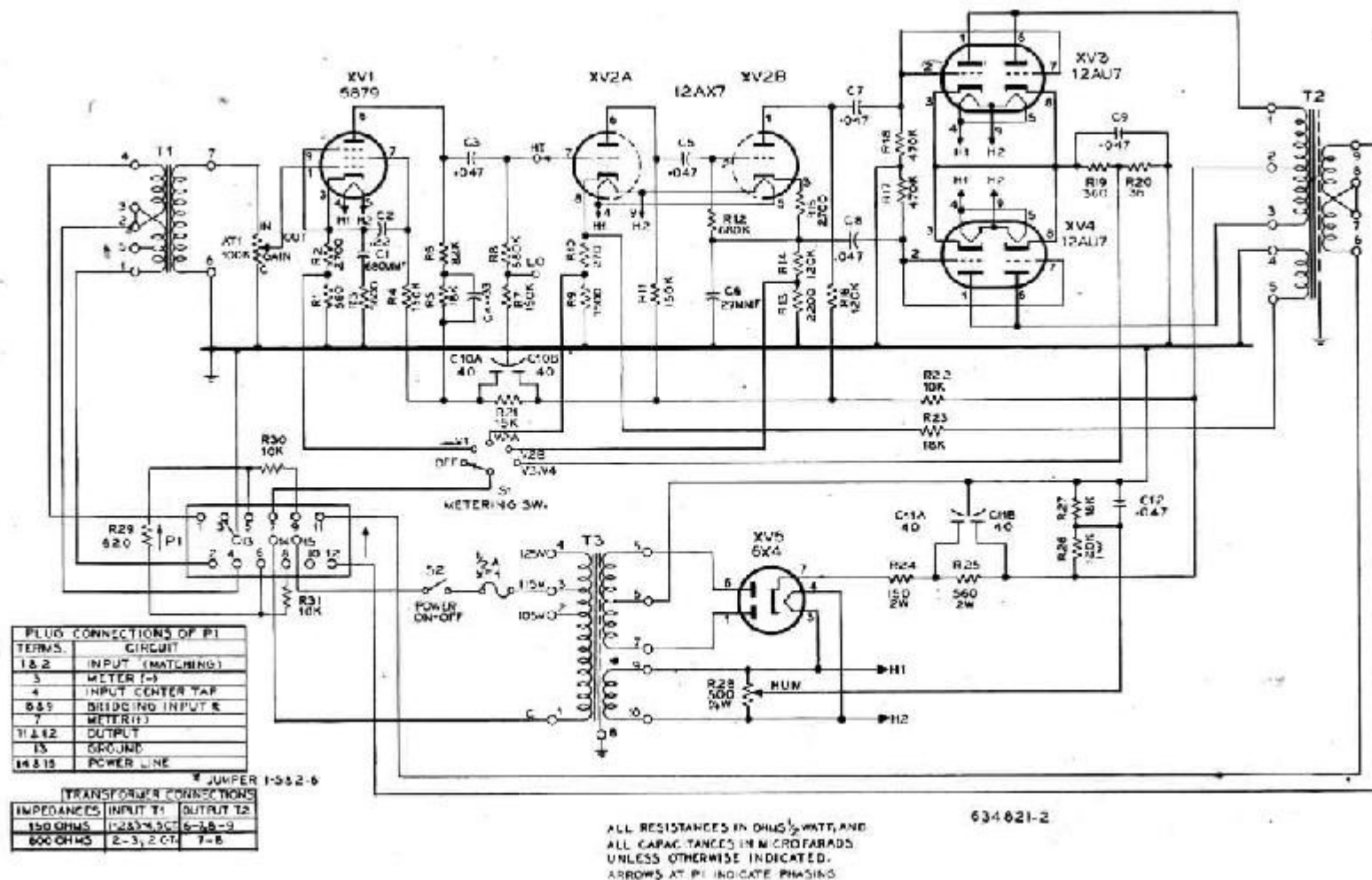
Figure 4 - Schematic Diagram
