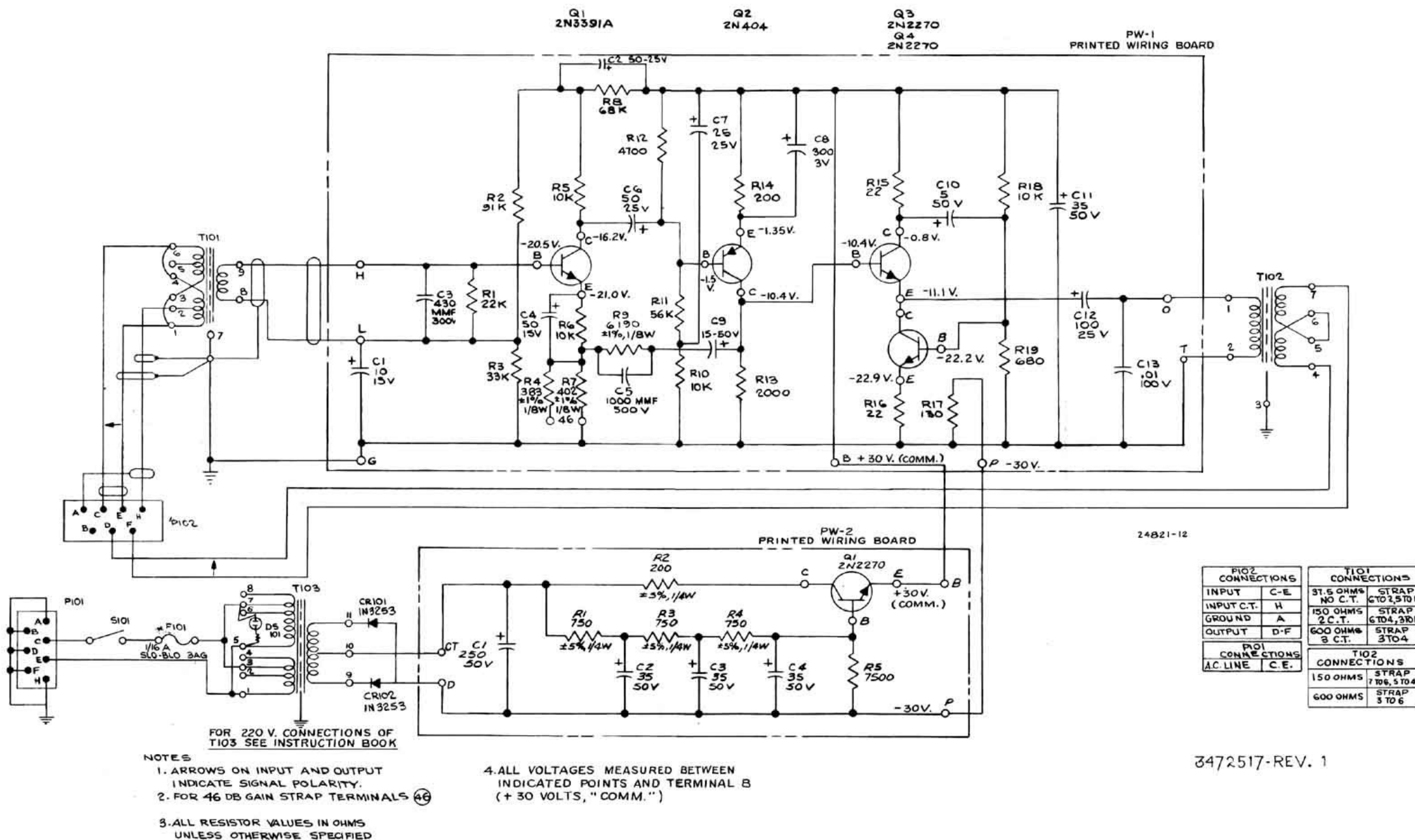
Figure 12—Schematic Diagram
