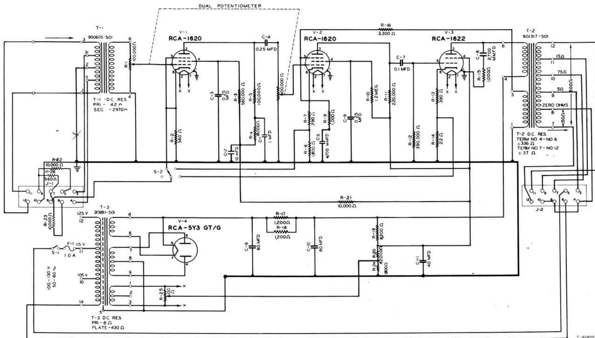
Figure 2—Schematic diagram of Type BA-3C Program Amplifier.
