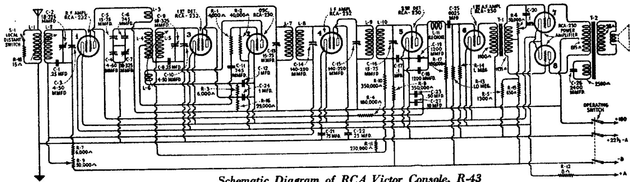
Schematic Diagram of RCA Victor Console, R-43
