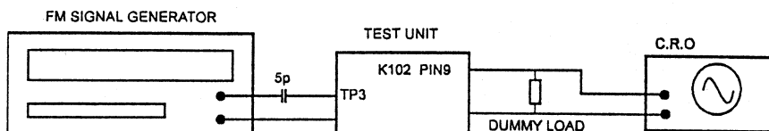
Figure 5. IF Alignment
