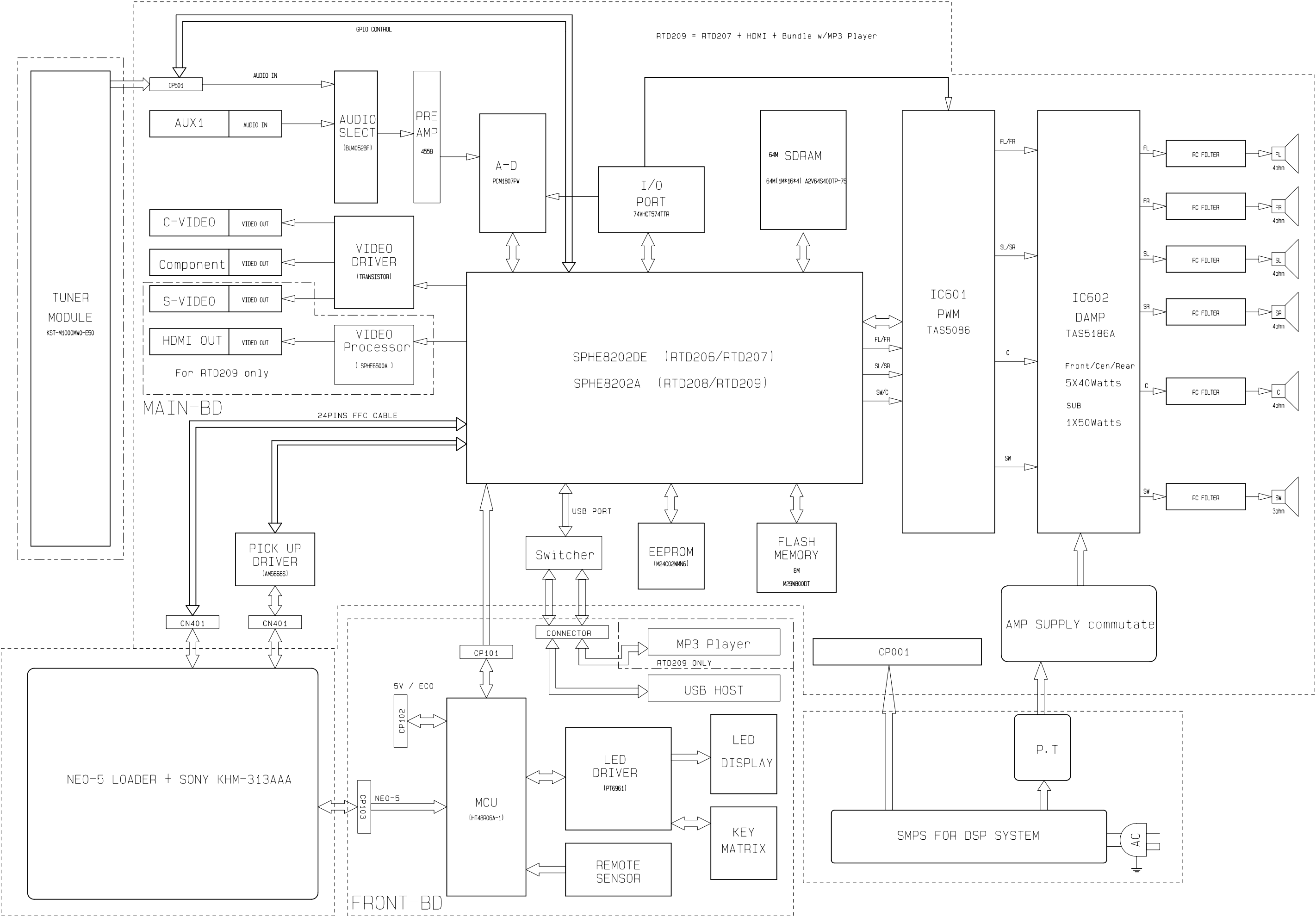
RTD207 Block Diagram
