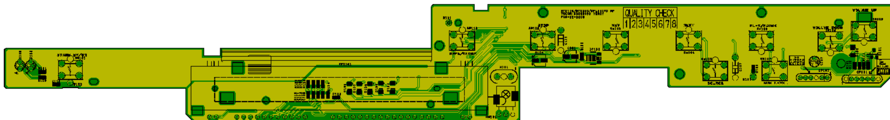
Front PCB (Top View)
