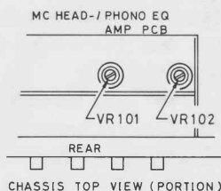
Fig. 1. Phono Amp DC Balance Adjustment
