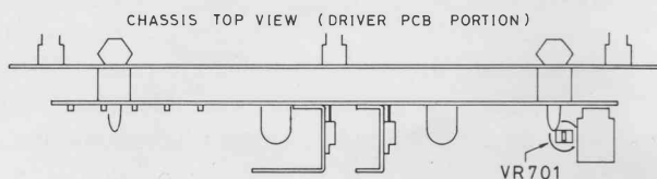
Fig. 2. Main Amp DC Balance Adjustment
