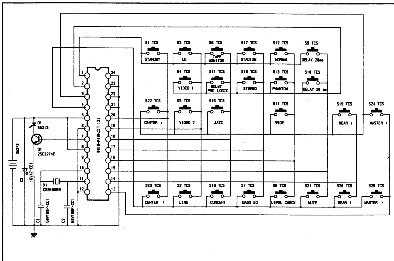
SCHEMATIC DIAGRAM MODEL RR-907
