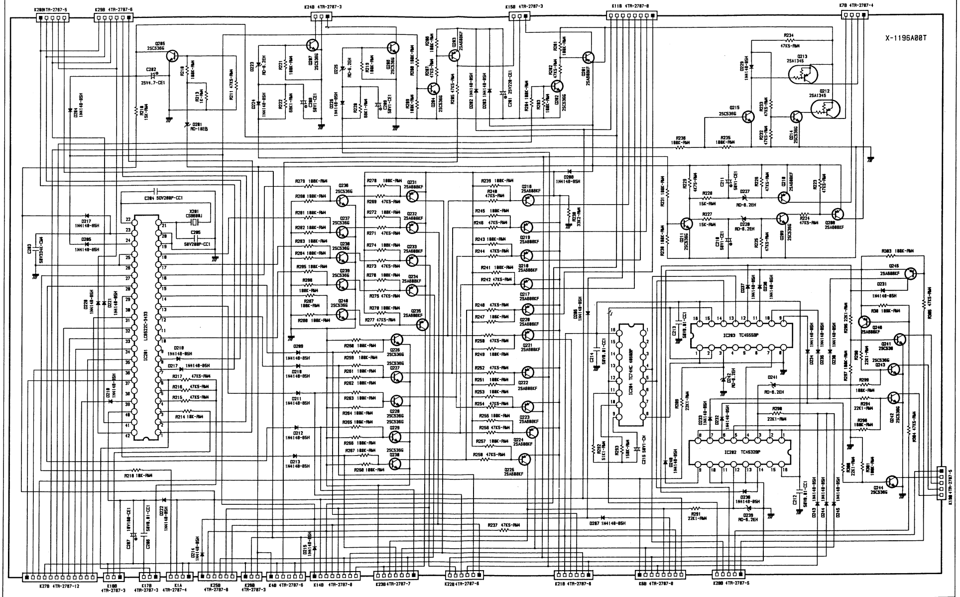
SCHEMATIC DIAGRAM RSP-960AX (2/4)
