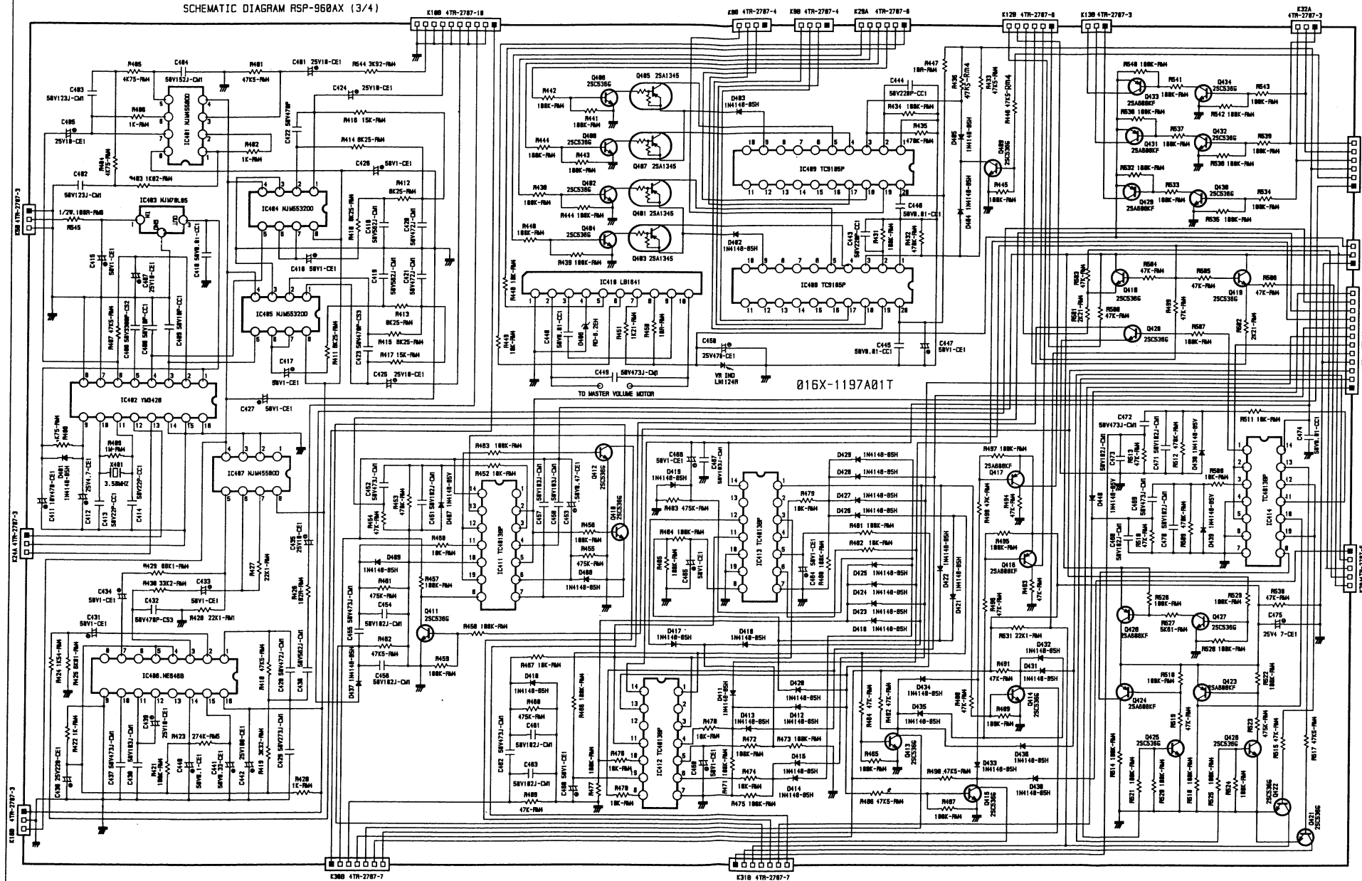
SCHEMATIC DIAGRAM RSP-960AX (3/4)
