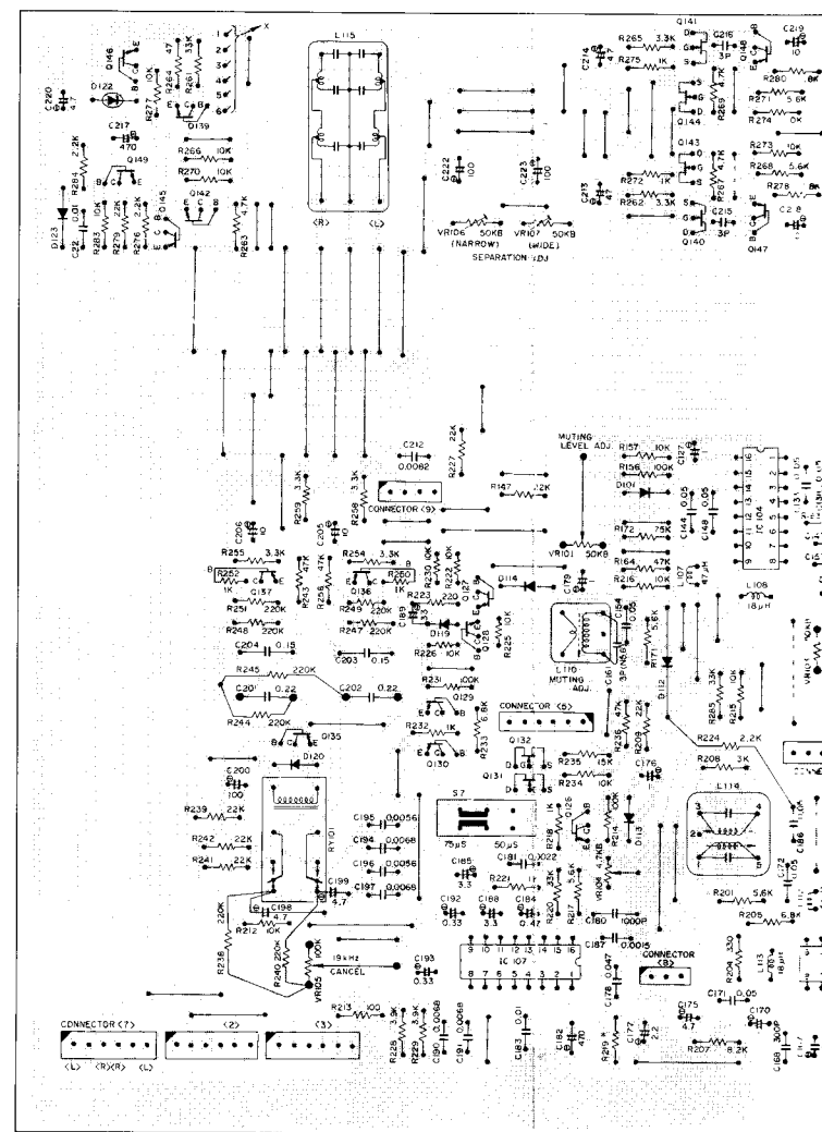
CONNECTOR (7) TO OUTPUT TERM. FIXED, VARIABLE CONNECTOR (2) TO POWER SUPPLY TO AM PCB CONNECTOR (3) TO LOCK IND DRIVER PCB CONNECTOR (4) TO LOCK IND DRIVER PCB CONNECTOR (5) TO FRONT END CONNECTOR (6) TO FRONT END
