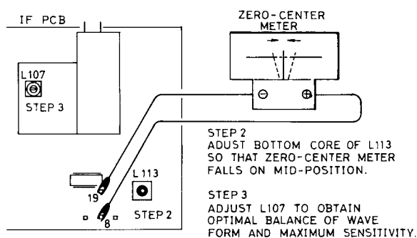
Fig. 1. FM IF Alignment
