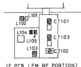
Fig. 2. FM RF Alignment
