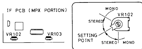
Fig. 5. FM Stereo Adjustment
