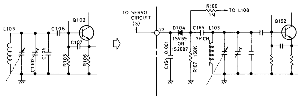
Fig. E FM OSC Circuit (Portion)
