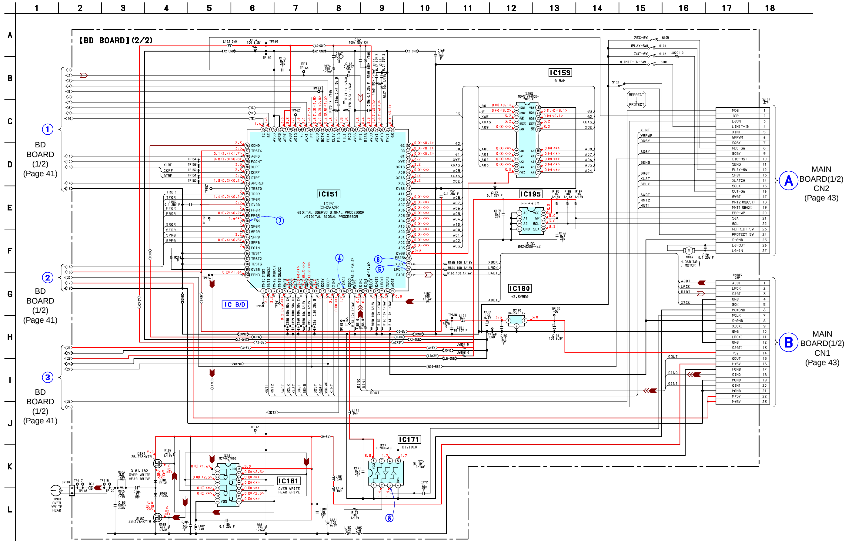
6-5. SCHEMATIC DIAGRAM – BD SECTION (2/2) – • See page 37 for Waveforms. • See page 53 for IC Pin Functions. • See page 50 for IC Block Diagrams.
