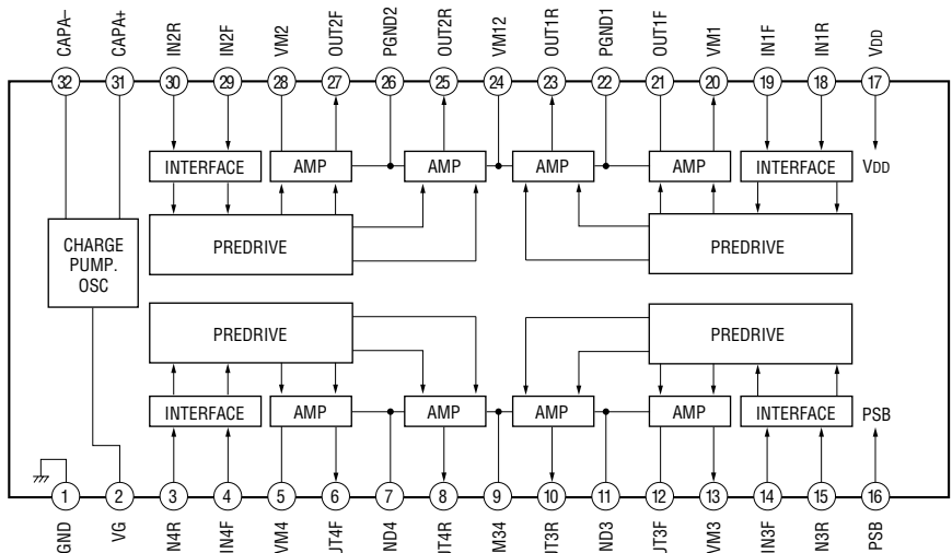
IC141 BH6511FS-E2 (BD BOARD)
