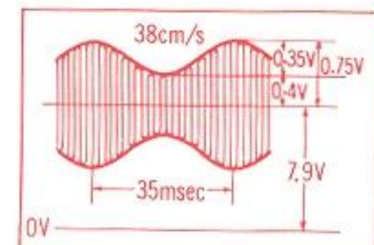
Position Detection Coil: Secondary
