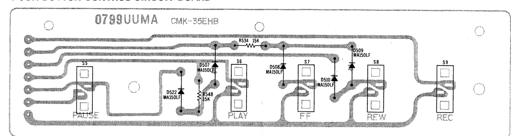
PUSH BUTTON CONTROL CIRCUIT BOARD
