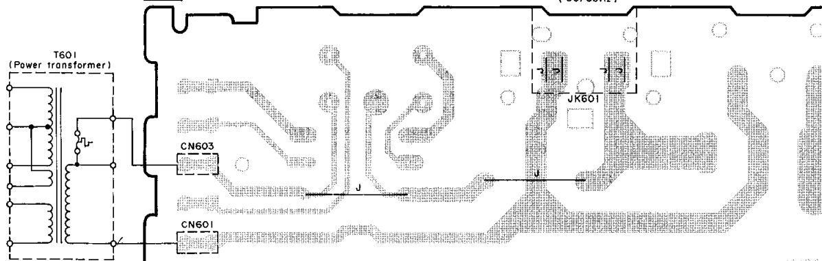
POWER SUPPLY P.C.B. (REP1806C-P)
