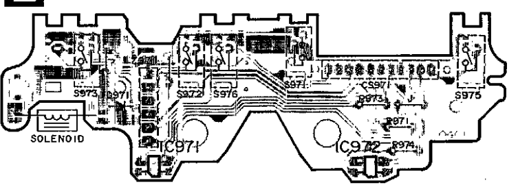
E MECHANISM P.C.B.(REP1954A)
