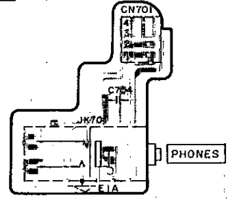
F HEADPHONES JACK P.C.B.(REP1957A-S)
