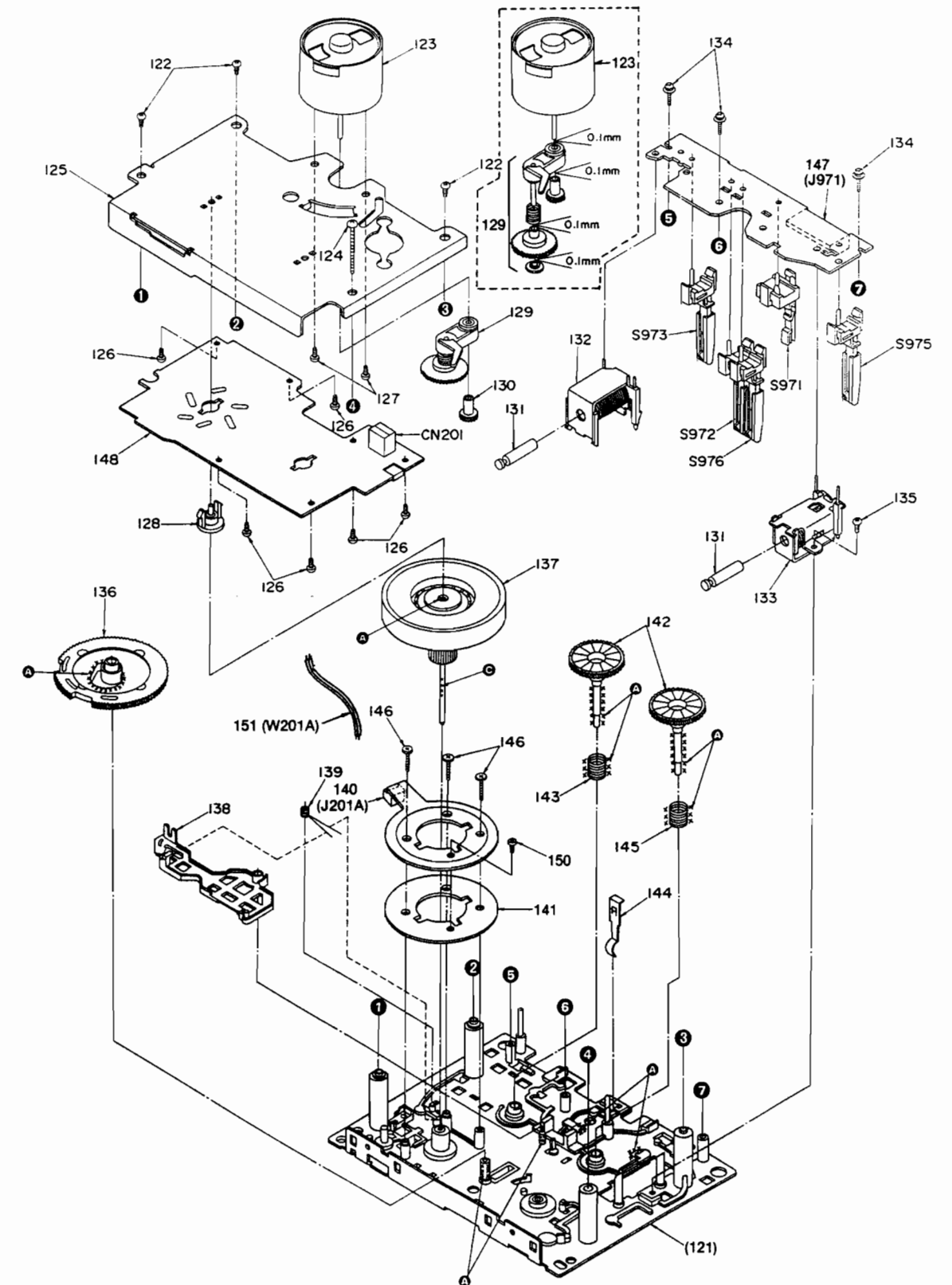
(Bottom view)
