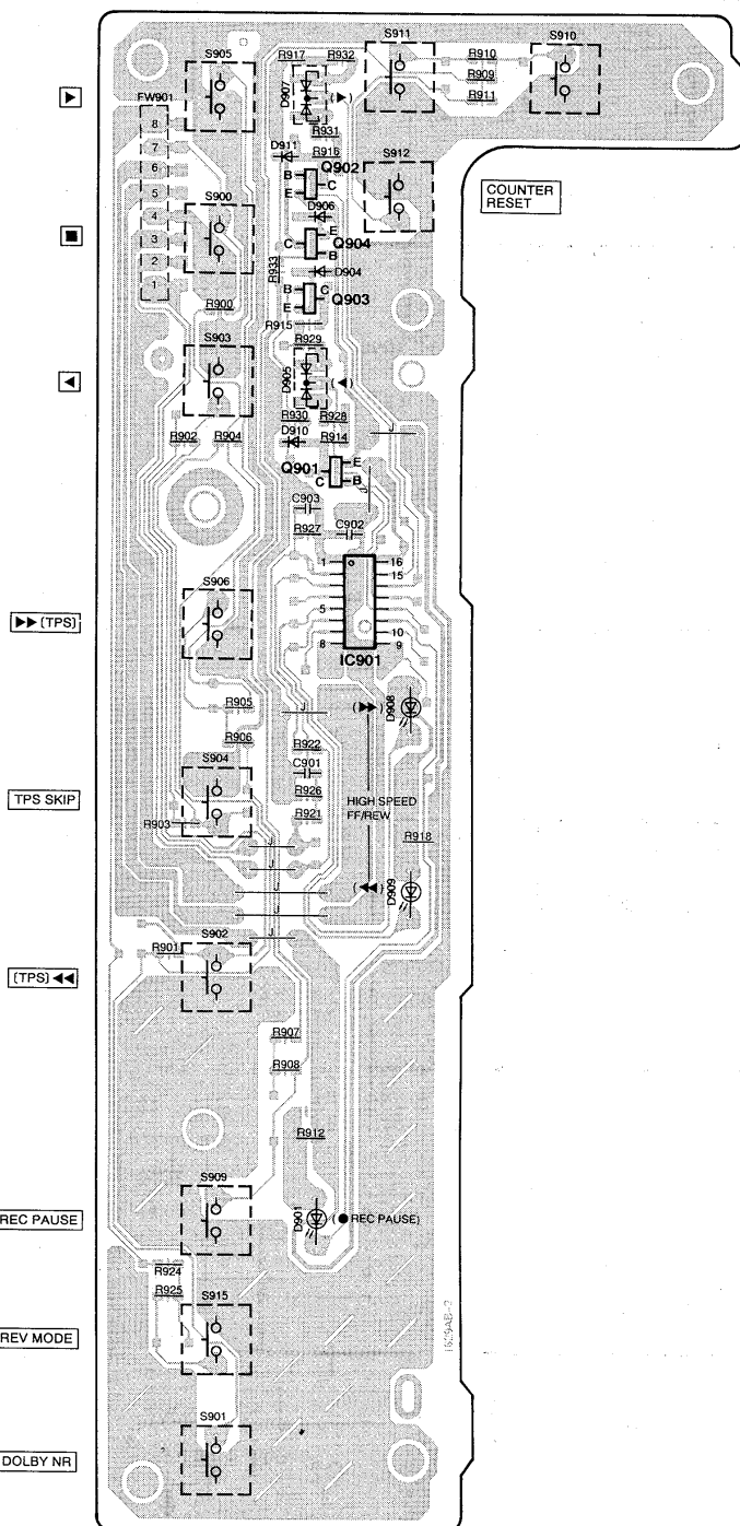
C OPERATION P.C.B. (REP2296A-2S)
