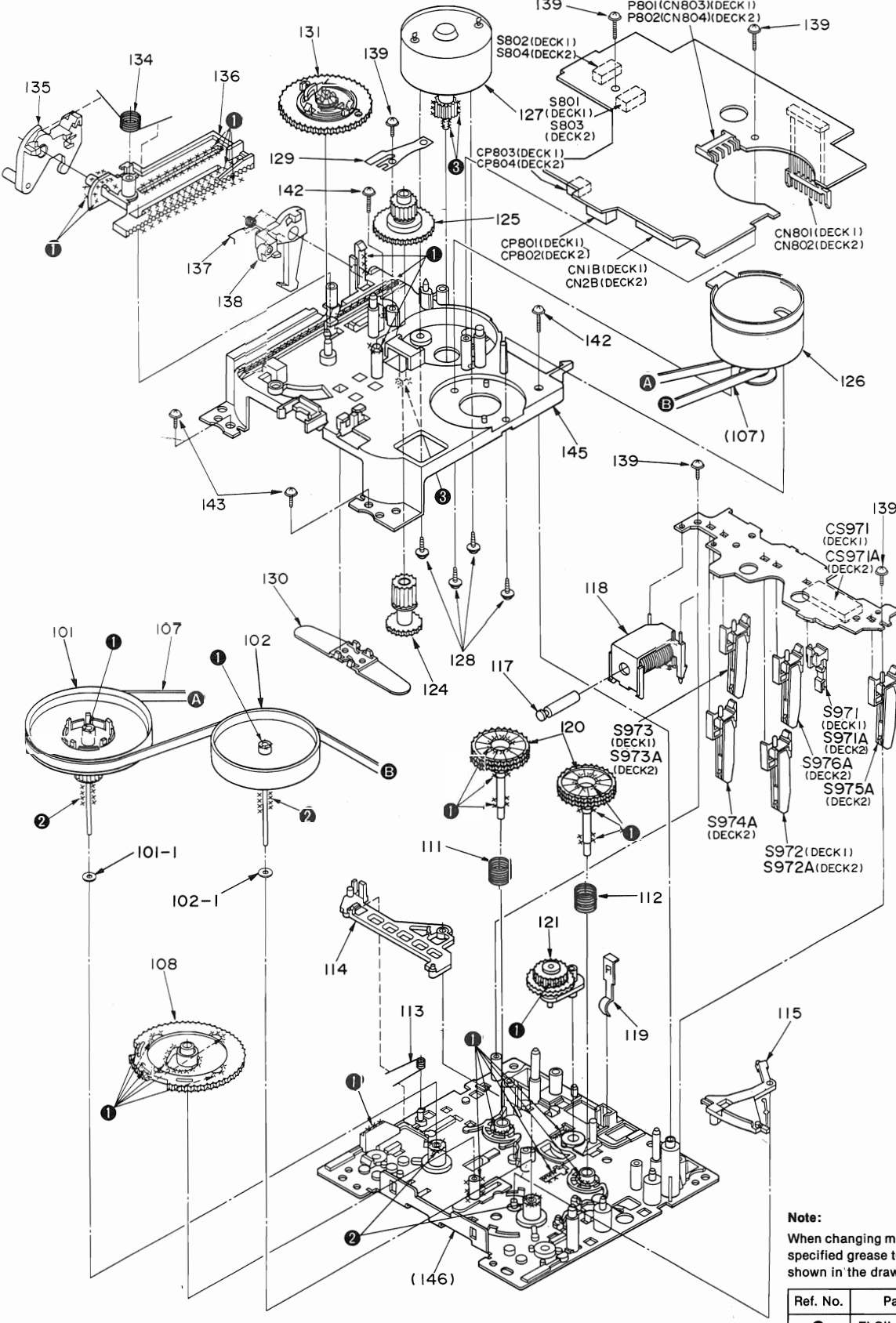
(Bottom view)
