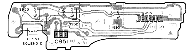
D MECHANISM ( DECK 2 ) P.C.B. ( REPO075 )
