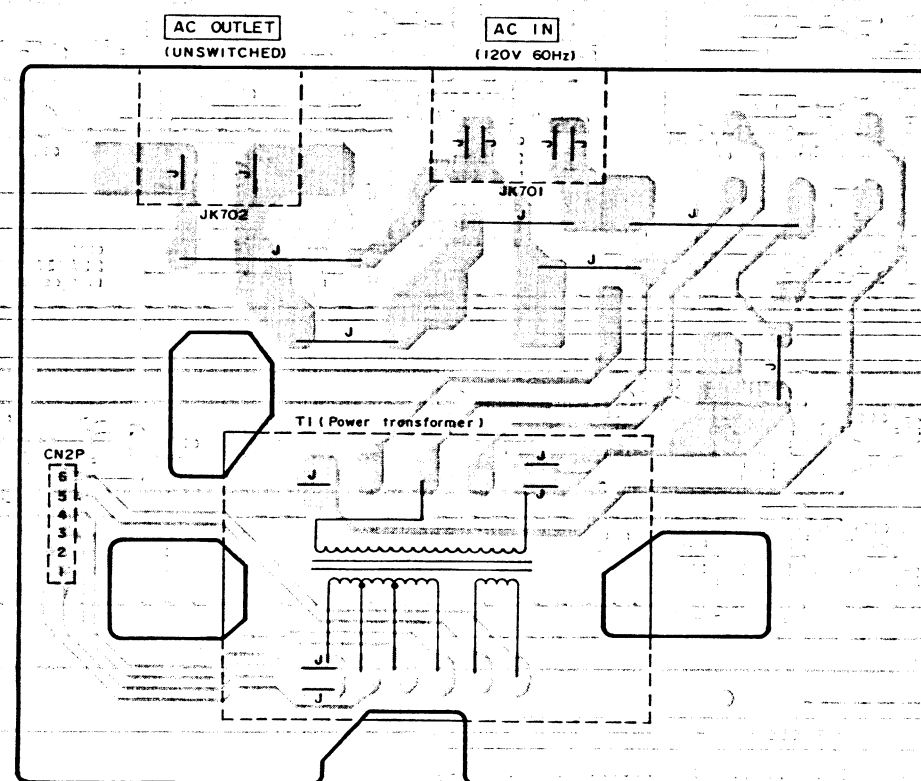
B POWER SUPPLY P.C.B. For [P,PC] areas.
