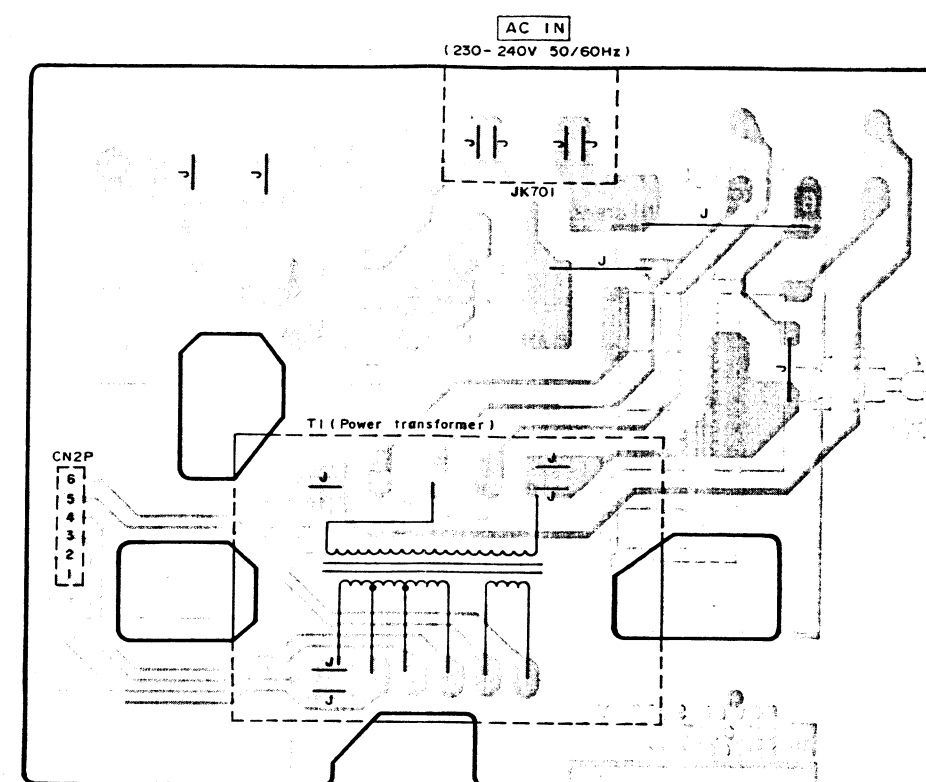
B POWER SUPPLY P.C.B. For [EB,EG,GN] areas.
