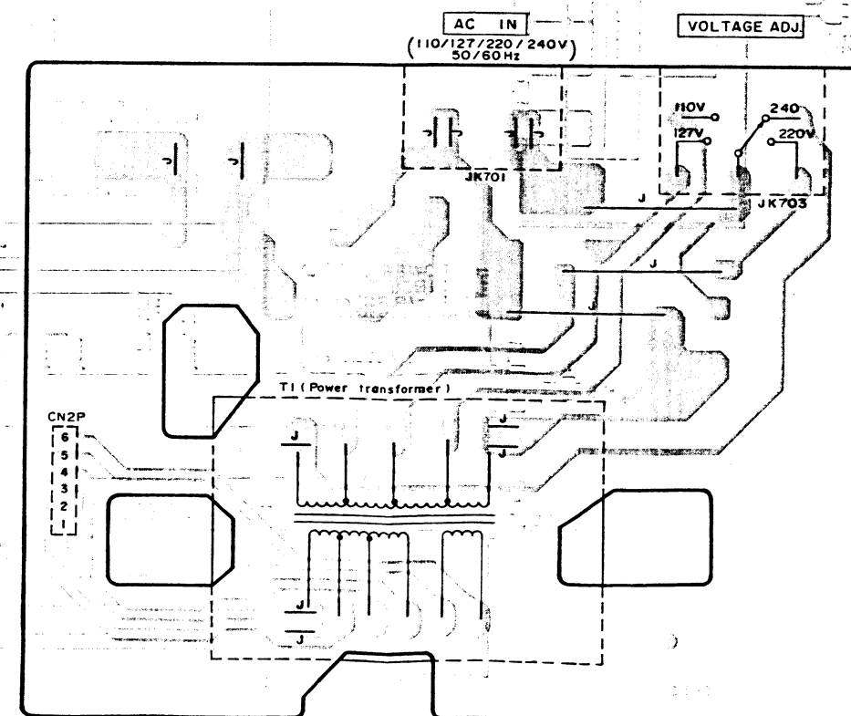
B POWER SUPPLY P.C.B. For [GC] area.
