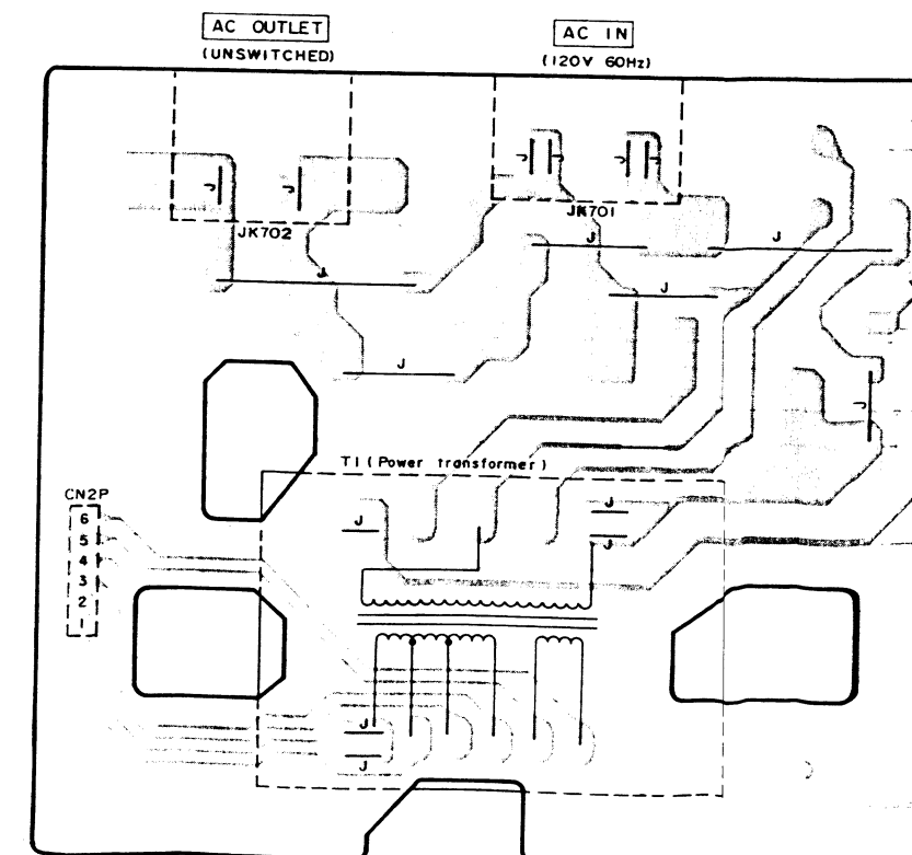
B POWER SUPPLY P.C.B. For [P,PC] areas.
